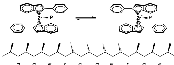
Scheme 2. “Oscillation” of a [(2-Ar-indenyl) 2 ZrCl 2 ]-based catalyst (shown for Ar = phenyl) between the two enantiomorphous forms of the rac -like conformation, and resulting polypropylene microstructure.
